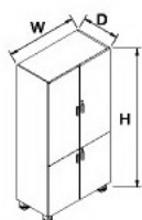
EXE文件高櫃 EXE-SI090180 W:900/D:470/H:1800mm
