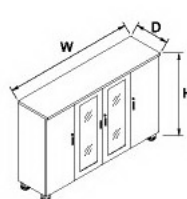
EXE中櫃 EXE-SZ180120 W:1800/D:470/H:1200mm
